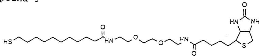
biotin compound 3
